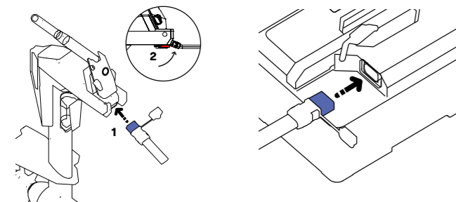
1 CONNECT OBM FIRST 2 CONNECT BATTERY AFTER
